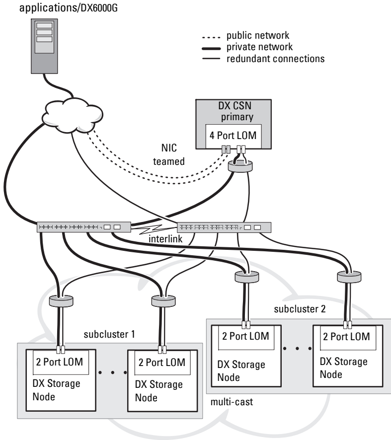
Figure 2-3. Subcluster Configuration
