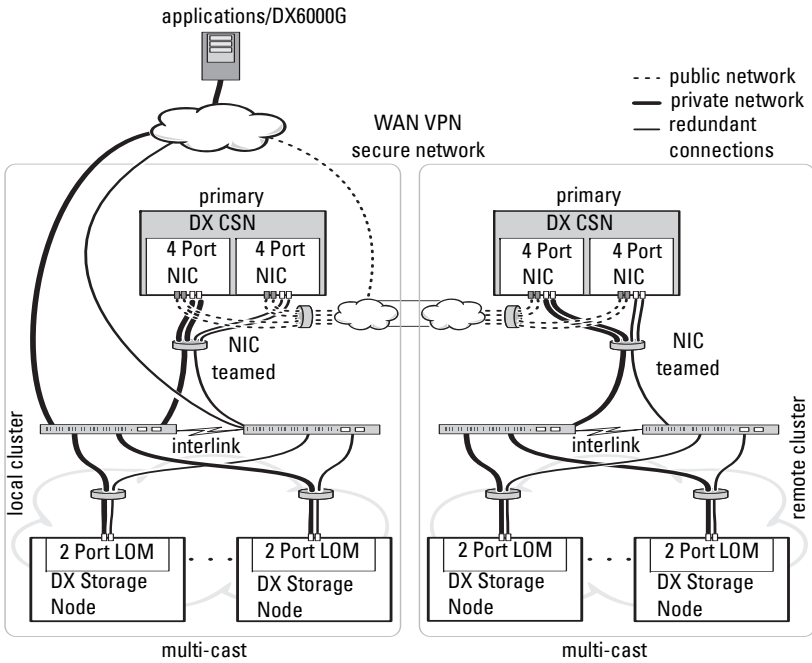
Figure 2-4. Multiple Cluster Configuration
