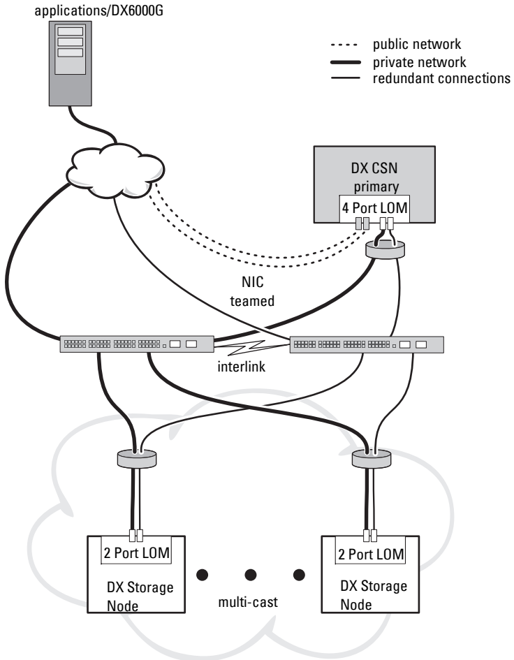
Figure 2-1. Local Cluster Configuration
