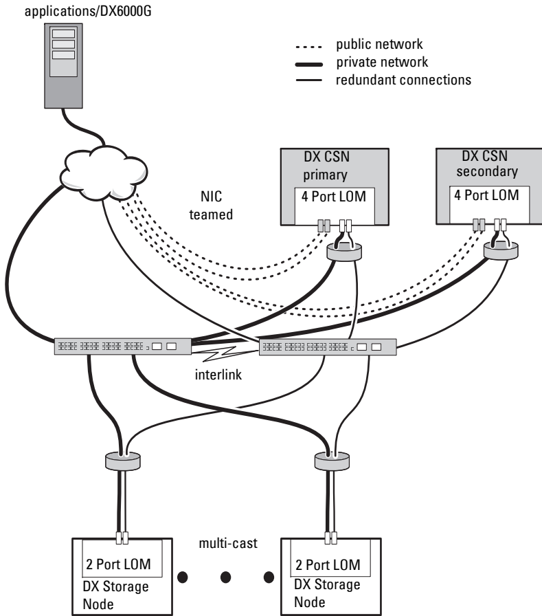
Figure 2-2. Redundant DX Cluster Services Nodes
