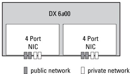
Figure 3-5. Ethernet Cable Connections to the External and Internal Networks
